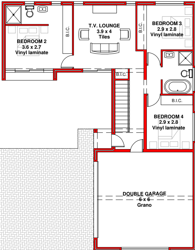
GROUND STOREY PLAN
