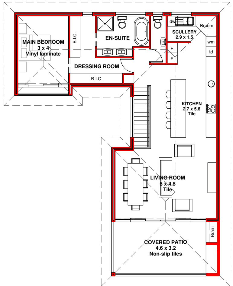
FIRST STOREY PLAN
