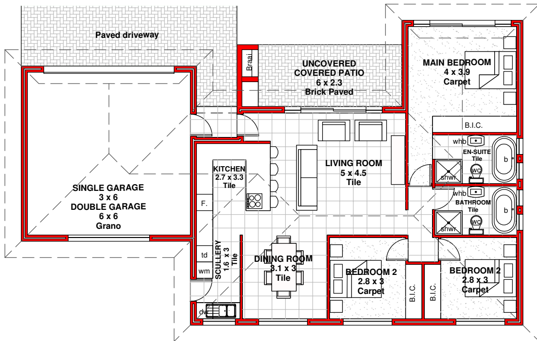
GROUND STOREY PLAN
