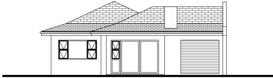
STREET ELEVATION
