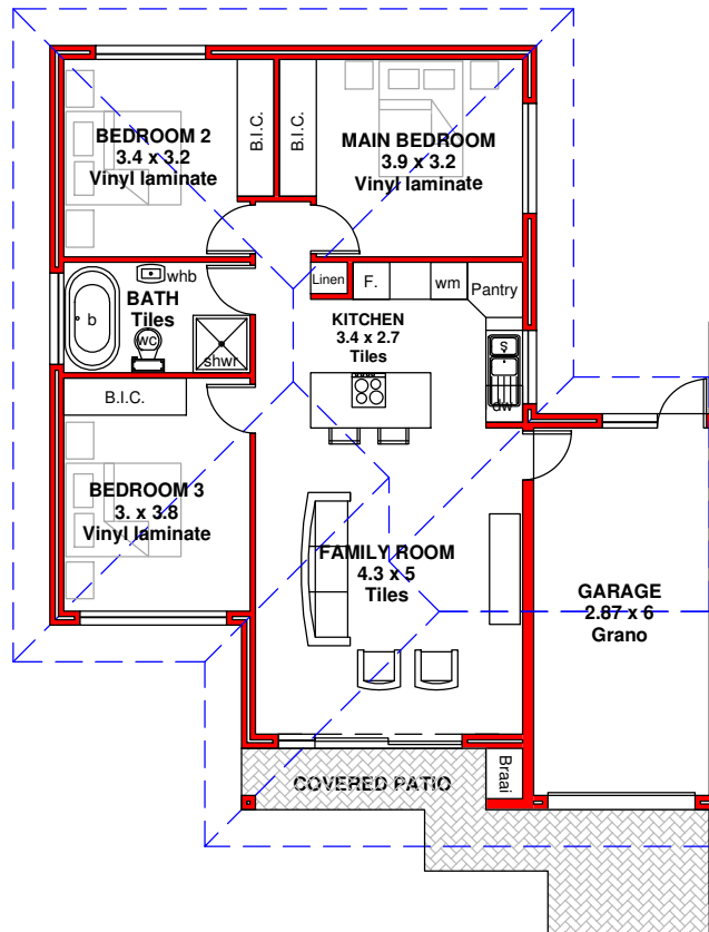
FLOOR PLAN
